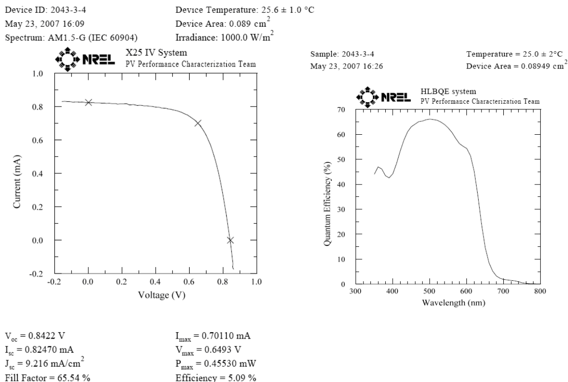
Figure 2: I-V and EQE spectrum of OPV device certified to 5.1% at NREL
