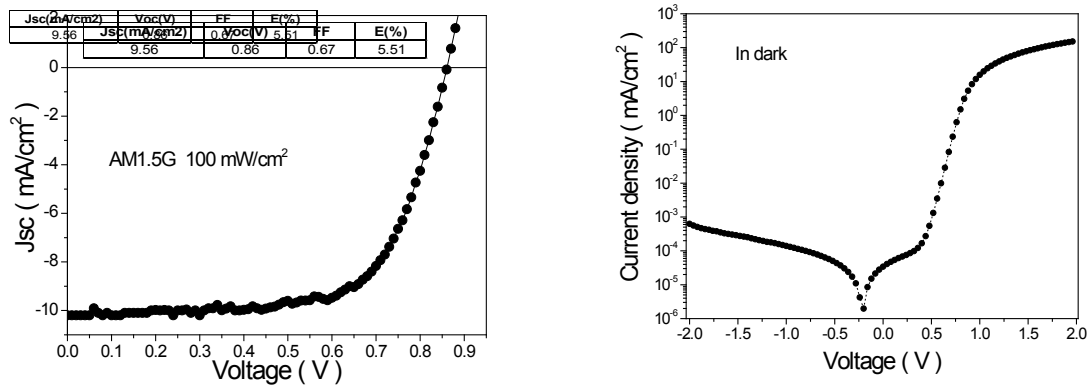
Figure 6: J-V characteristics of device under AM1.5G 100 mW/cm 2 (left) and in dark (right).
