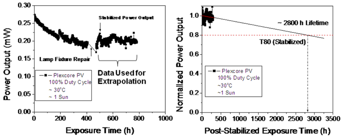
Figure 20:(left): The output power of a device under ~1sun changes with time. The temperature of the substrate was controlled at ~30°C; (right): Normalized output power changes with time after the output power stabilized
