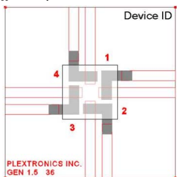
Figure 1: Plextronics' lab-cell design
