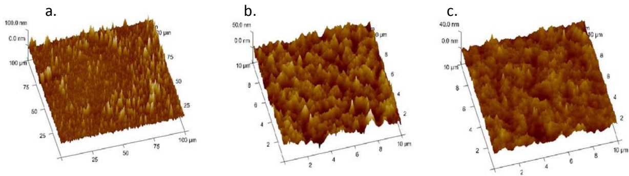
Figure 30: AFM profile of sprayed HIL film with thickness around 50nm at different dilution ratio (a) HIL:MeOH=1:5, R(rms)= 11nm, R(peak to valley)= 128nm, (b) HIL:MeOH:IPA=1:4:1, R(rms)= 7nm, R(peak to valley)= 74nm, (c) HIL:MeOH:H 2 O=1:0.5:3.5, R(rms)= 4nm, R(peak to valley)= 36nm.
