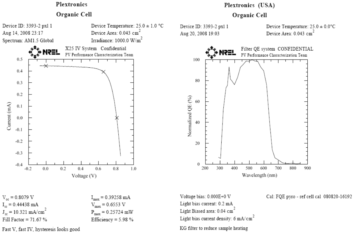
Figure 35 (left): I-V data of OPV device certified to 5.98% at NREL; (right): Normalized EQE spectrum
