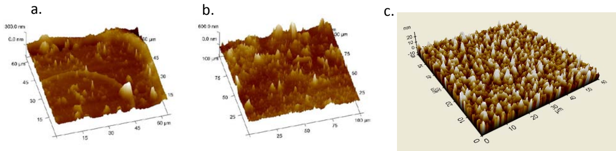
Figure 31: AFM profile of spray coated OPV active material for different solvent mixture (a) A:B=1:2, R(rms)= 45nm, (b) A:B:C=1:2:1, R(rms)= 87nm, (c) D:B =1:1, R(rms)= 4nm.
