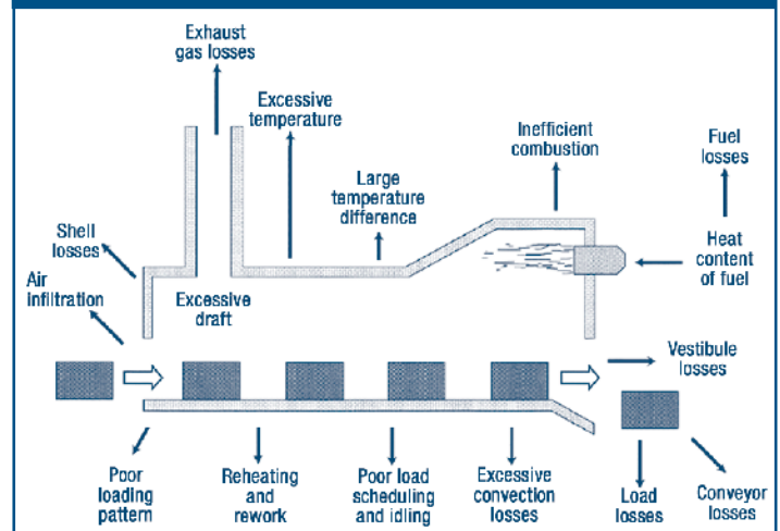
Figure 2. Heat losses
