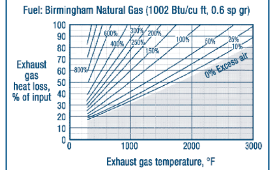
Figure 1. Heat in flue gas
