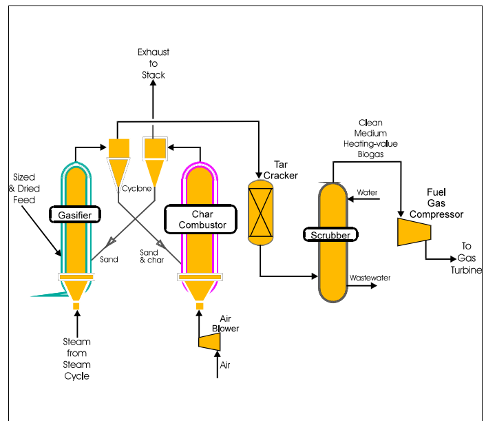
Figure 5.4: Indirect Gasifier
