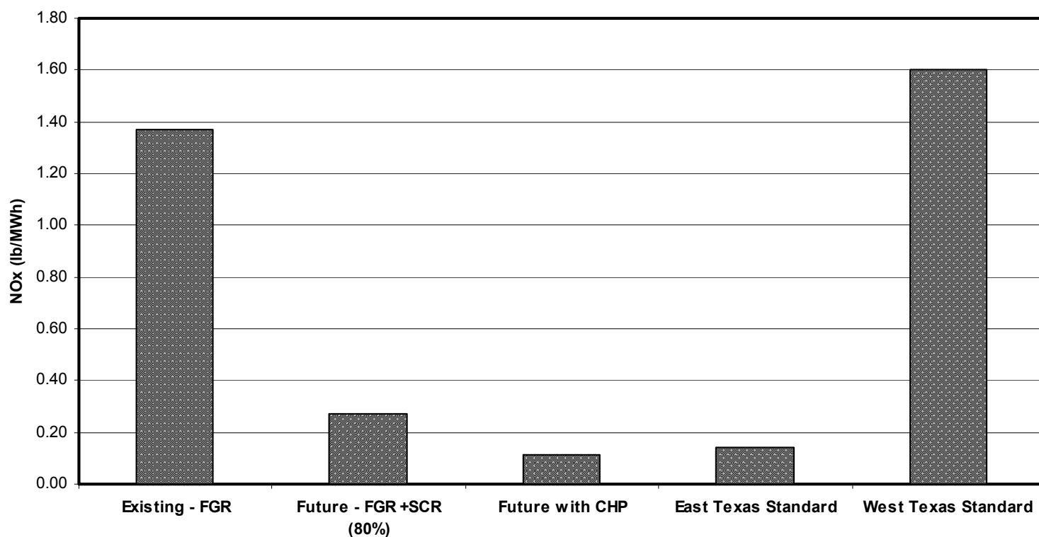
Figure 6.3: Biomass Combustion - Potential for NO x Reduction
